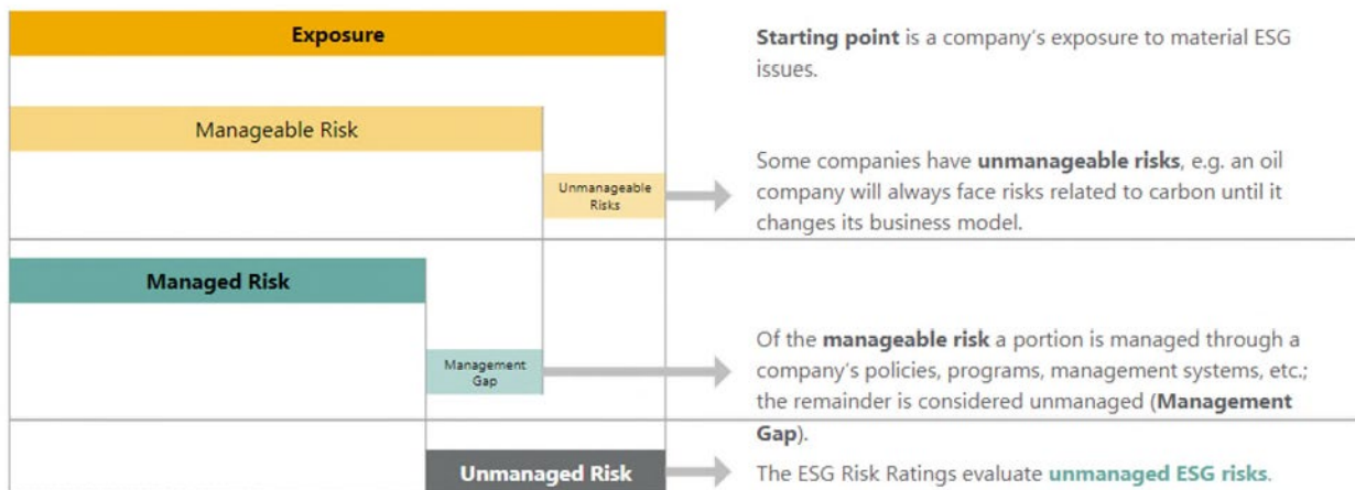
Exhibit 2: Risk decomposition
